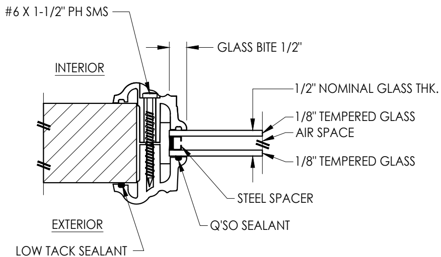
G1 GLAZING DETAIL Lip Lift Insert Glazing
